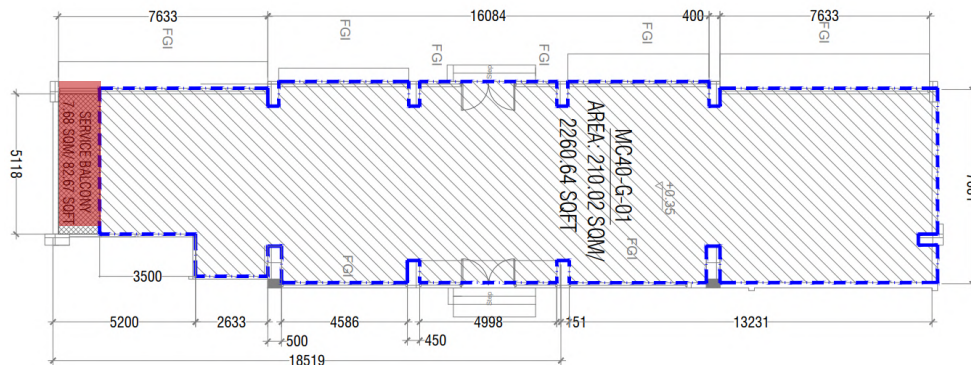
Figure 1: AC Outdoor unit locations marked in red (must be placed at ground floor level at a level higher than 300mm from finished ground floor level).
