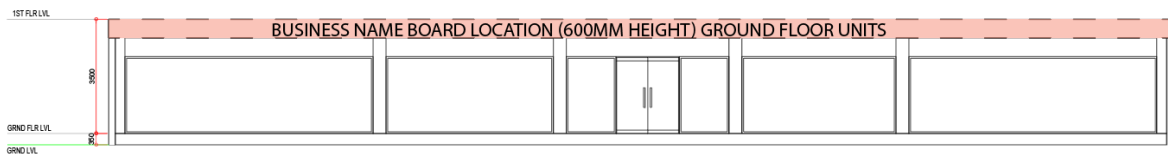
Figure 2: Commercial frontage Elevation with business name board location and dimensions.
