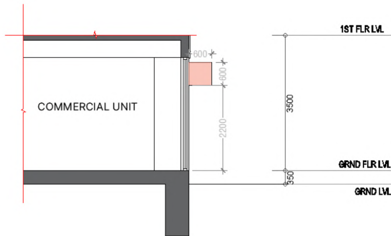
Figure 3: Commercial side elevation with business name board and logo location.
