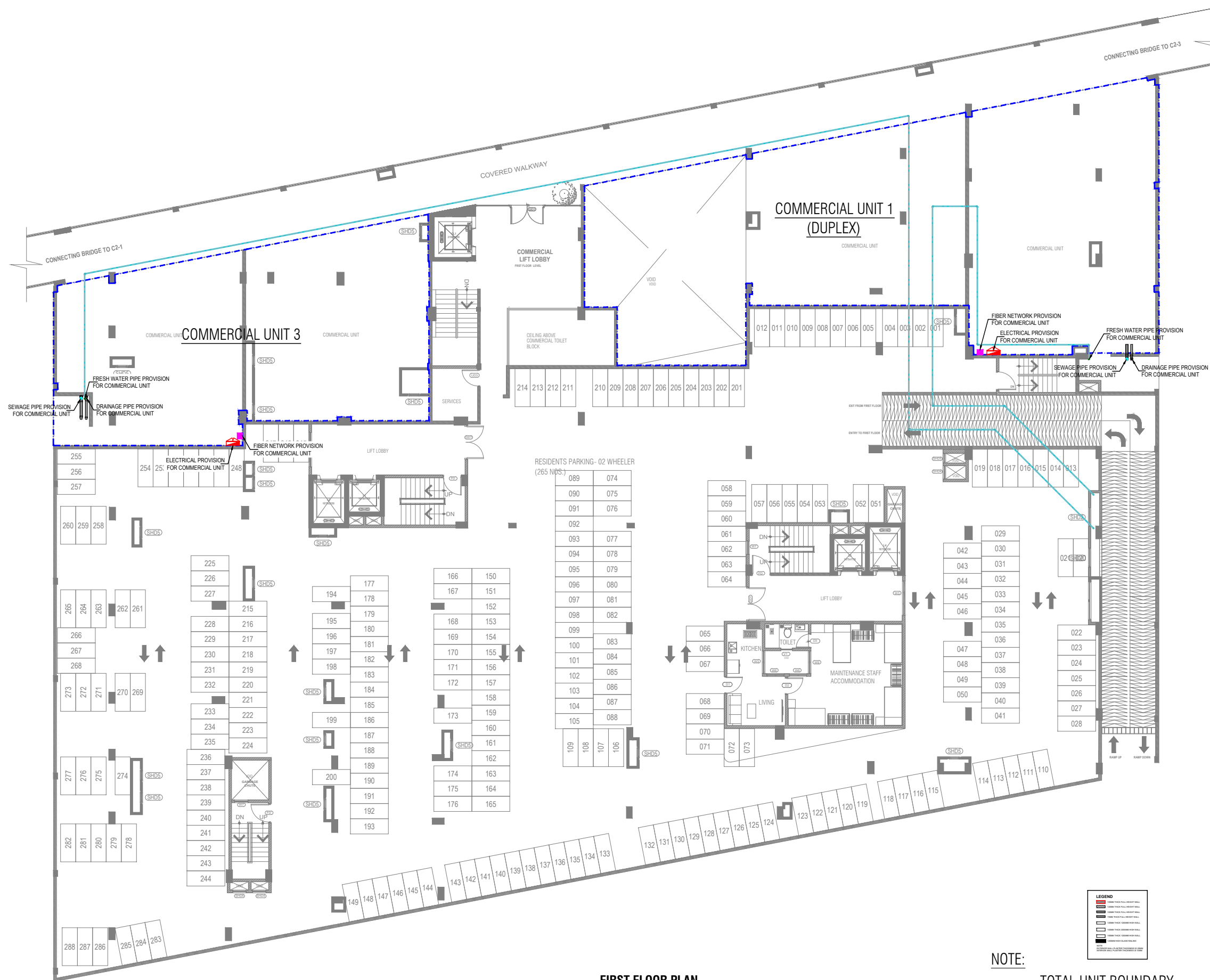
FIRST FLOOR PLAN SCALE 1:150
